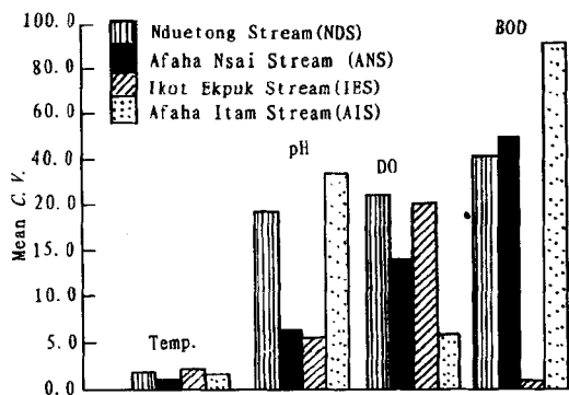
Fig.2 Coefficients of variation of oxygen and related variables in the samples
