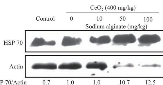
Fig. 5 Effects of CeO 2 NPs plus alginate on HSP 70 expression in corn leaves estimated by Western blot analyses. Equal amounts of total protein extracts (20 \mu g) from leaves were loaded in each lane. Protein blots were probed with primary antibodies directed against HSP 70. Total tissue protein was fractionated by SDS-PAGE, transferred to membranes, and probed with HSP 70 antibodies. The expression level of HSP 70 was normalized to actin and fold of change was measured by densitometry.
