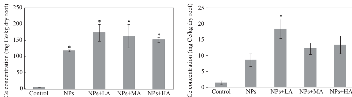
Fig. 1 Cerium concentration in (a) roots and (b) shoots of corn plants (Golden variety) grown for one month in a farm soil. The soil was treated with 400 mg/kg CeO 2 NPs and alginate at 10 (LA), 50 (MA) and 100 (HA) mg/kg soil. Error bars stand for standard deviation. * Stands for statistic differences at p < 0.05 . LA, MA, and HA represents low, medium, and high alginate.
