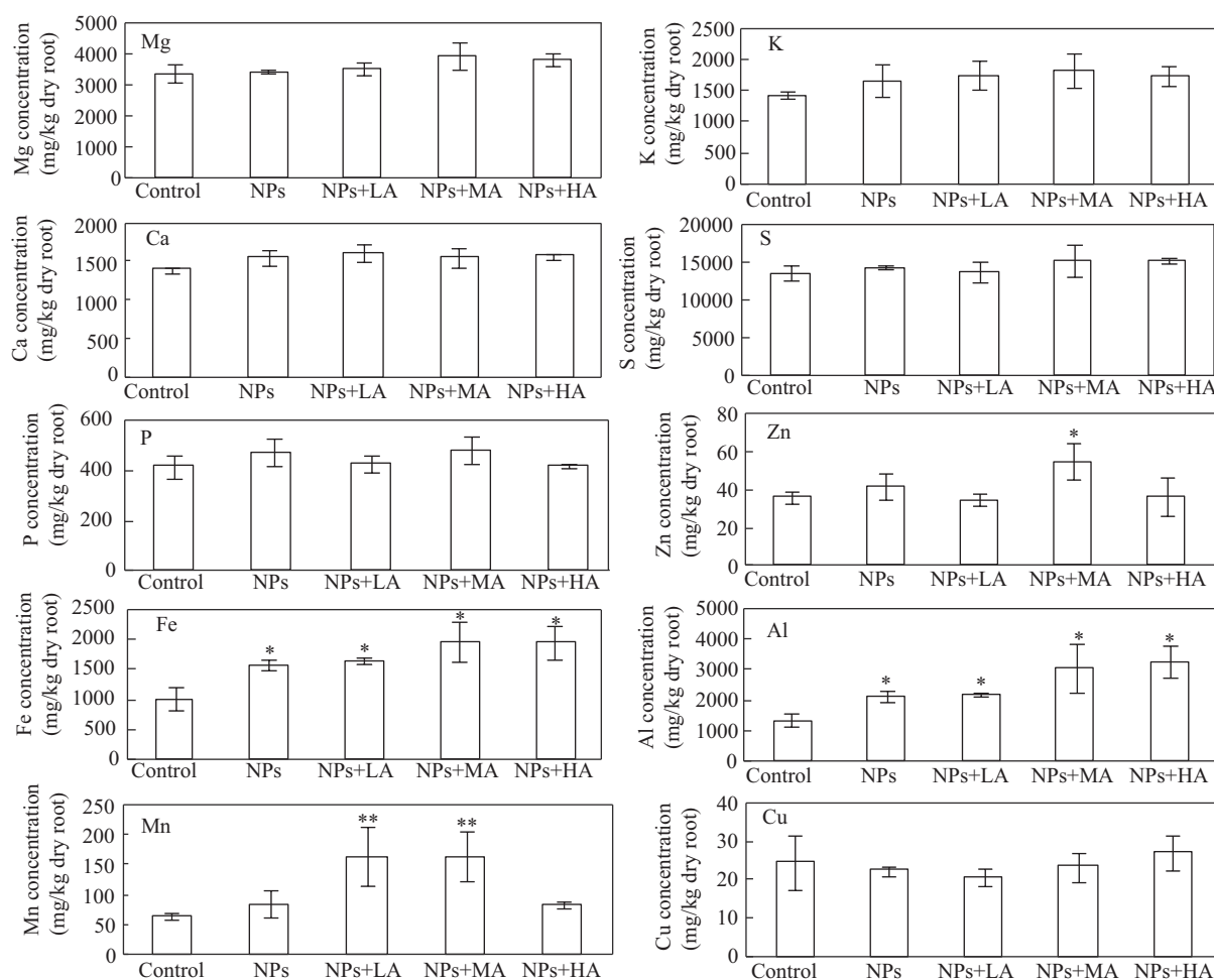
Fig. 2 Micro and macro nutrient contents in roots of corn plants grown for one month in a farm soil. The soil was treated with CeO 2 NPs with different concentration of alginate. Error bars stand for standard deviation. ** Stands for statistic differences at p < 0.01 ; * stands for statistic differences at p < 0.05 .
