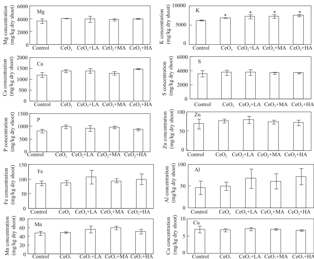
Fig. 3 Micro and macro nutrient contents in shoots of corn plants grown for one month in a farm soil. The soil was treated with CeO 2 NPs with different concentration of alginate. Error bars stand for standard deviation. * Stands for statistic differences at p < 0.05 .
