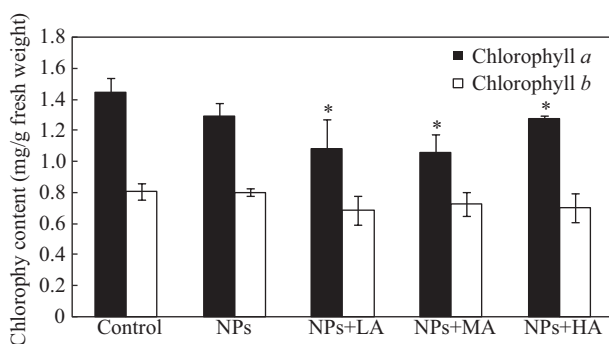
Fig. 4 Content of Chlorophyll in corn leaves grown for one month in a farm soil. The soil was treated with CeO 2 NPs with different concentration of alginate. Error bars stand for standard deviation. * Stands for statistic differences at p < 0.05 .
